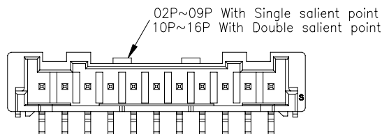
10P-16P SCALE 0.8:1
