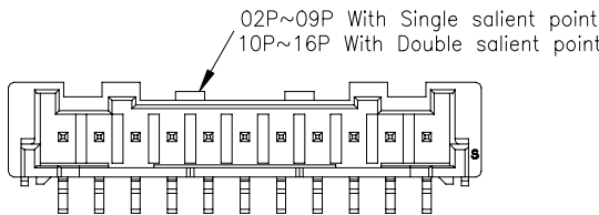
10P-16P SCALE 0.8:1
